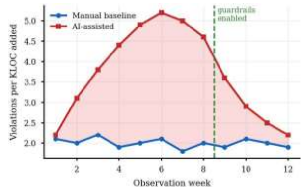
Fig. 3. Architectural conformance violations per KLOC added over the 12-week observation window, before and after automated guardrails were enabled. Values are the team's aggregated weekly telemetry; we did not independently re-derive them from raw logs.
