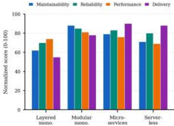
Fig. 2. Normalized quality scores of the four single-implementation reference builds (0–100 within this set of four; descriptive, n = 1 per style).
