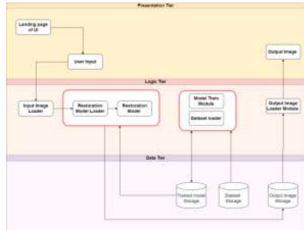
Figure 4. Proposed three-tier system architecture for deploying the framework.
