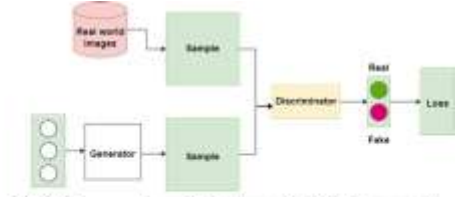
Figure 2: Structure of GAN (Self composed)
