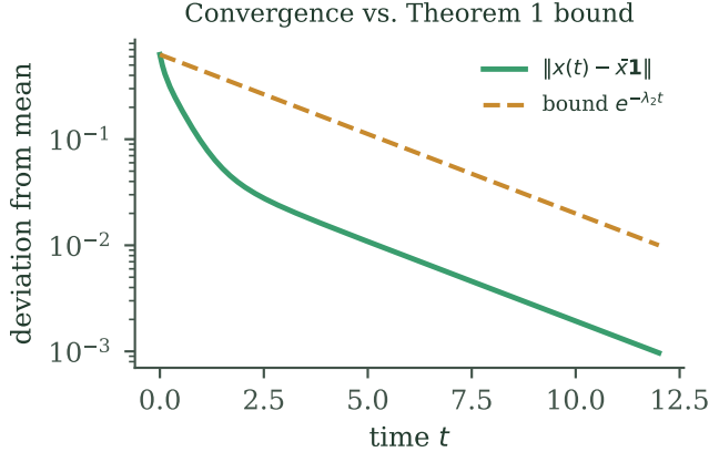
Fig. 5. Observed convergence of \|x(t) - \bar{x}\mathbf{1}\| against the theoretical bound of Theorem 1.
