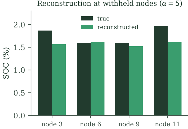
Fig. 4. True vs. reconstructed SOC at the four withheld nodes.
