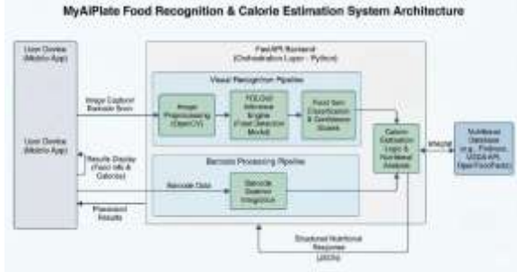
Fig. 2. Architecture diagram for AI processing – MyAiPlate Mobile Application
