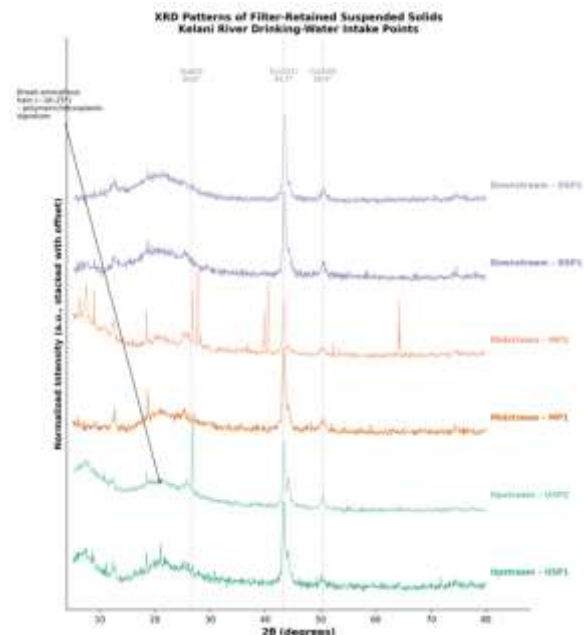
Figure 4 : XRD graph image take from Kelani River 6 water samples
