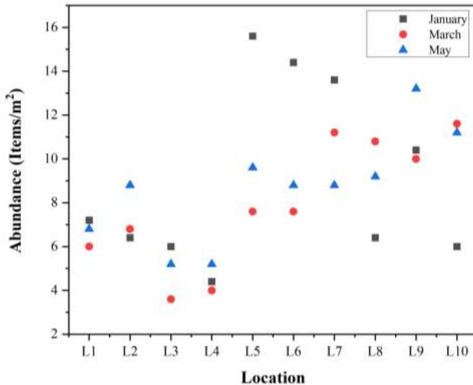
Figure 4. Spatial distribution of macro-litter abundance (items/m 2 ) across the sampling location
