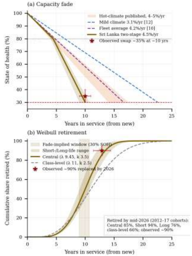
Figure 3. C1 (Leaf 24 kWh) validation: (a) capacity fade, theoretical vs. Sri Lankan; (b) Weibull retirement vs. fade model and field evidence.
