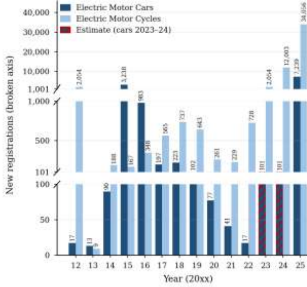
Figure 1. Electric vehicle registrations used in the model, Sri Lanka, 2012–2025 (broken axis).
