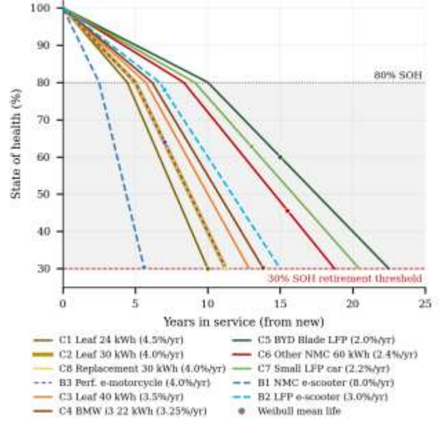
Figure 2. Illustrative capacity fade of all pack models in Sri Lankan conditions (central rates); dots mark Weibull mean life from new.
