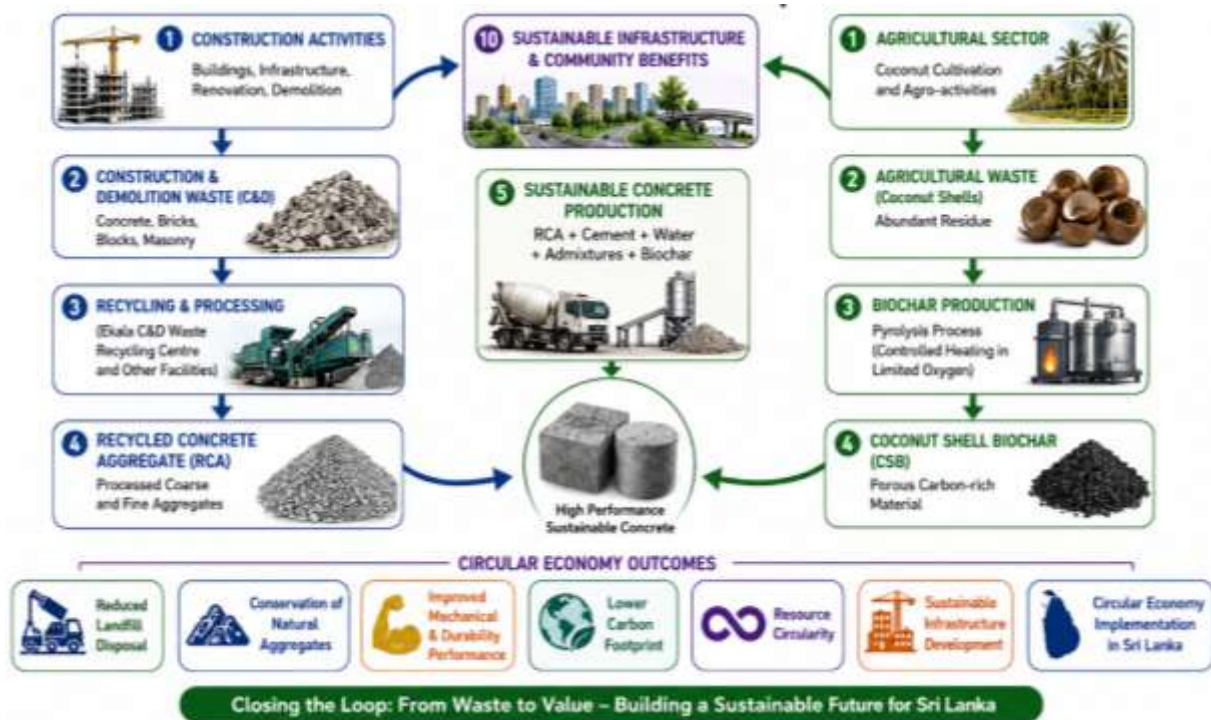
Figure 2. Proposed Construction–Agriculture Circular Resource Loop Framework for Sri Lanka
