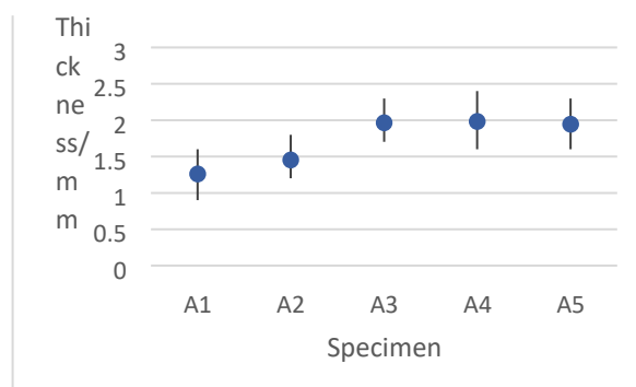
Figure 4 Effect of nutmeg shell powder concentration on the thickness of corn starchbased bioplasic films
