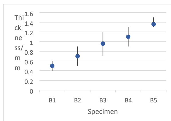
Figure 5 Effect of nutmeg shell powder concentration on the thickness of agar-based bioplasic films
