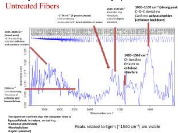
Figure 6 : FTIR spectrum of untreated fibre
