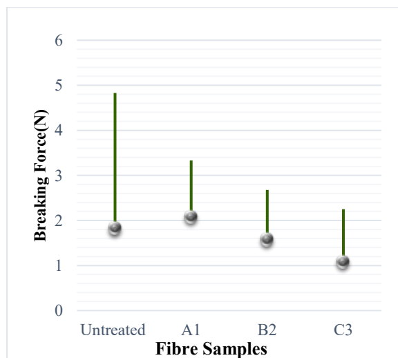
Figure 4 : Breaking force of untreated and chemically treated fibre
