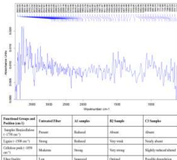
Figure 7 : FTIR spectrum of C3 sample treated fibre
