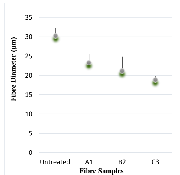
Figure 5 : Fibre diameter of untreated and chemically treated fibre
