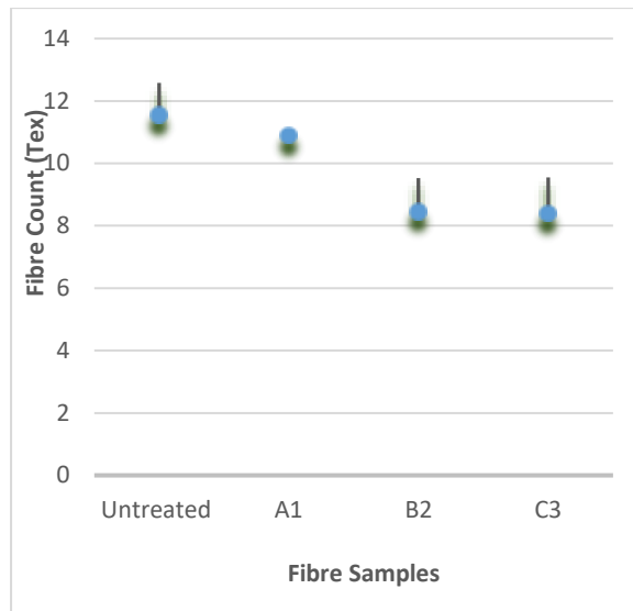
Figure 3 :Fibre count of untreated and chemically treated fibre
