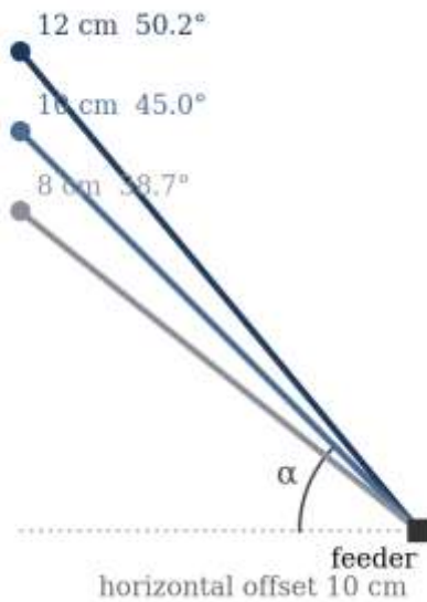
Figure 1. The three feeding-angle configurations, drawn to scale.
