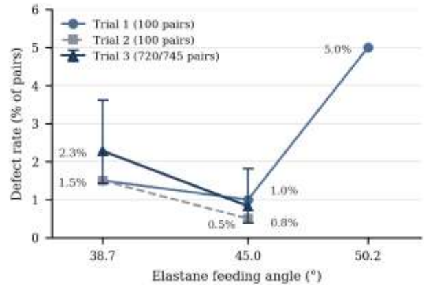
Figure 2. Elastane defect rate by feeding angle, all three trials. Error bars show 95% confidence intervals for Trial 3.
