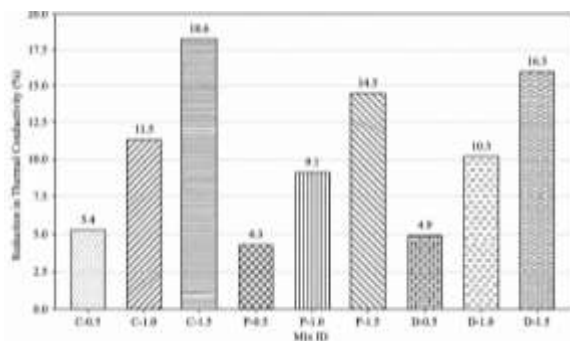
Figure 5. Thermal Conductivity results
