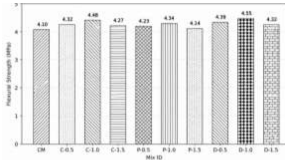
Figure 4. Flexural Strength results
