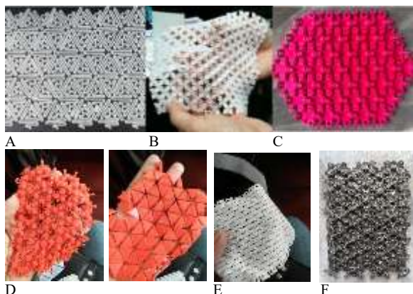
Figure 5. Sample testing using different filaments: A – TPU, B – PLA, C – ABS, D – PLA, E – PLA, F – Nylon.
