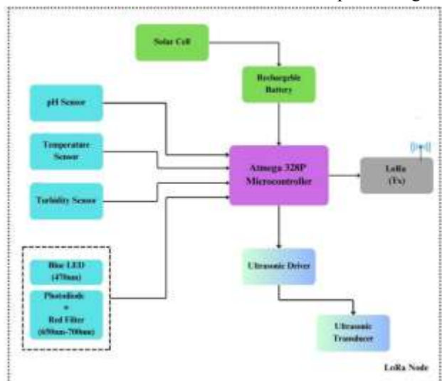
Fig. 1. Block-level architecture of the proposed HAB monitoring and mitigation buoy.
