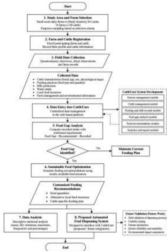
Figure1. Research Workflow of the Proposed CattleCare Framework
