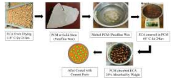
Figure 1. PCM integration process.
