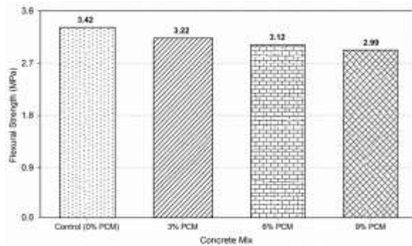
Figure 4. Flexural strength performance
