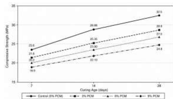
Figure 3. Compressive Strength Performance
