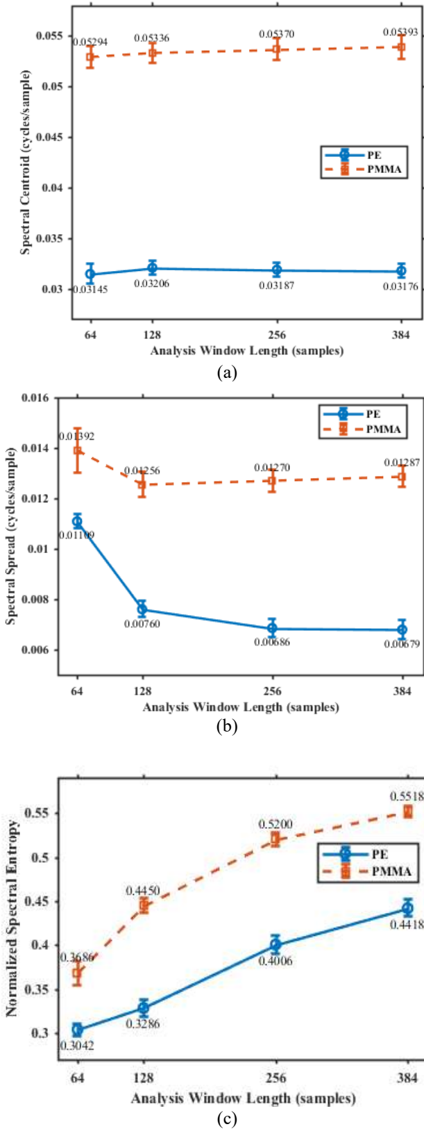
Figure 2. Effect of echo-analysis window length on group-level spectral features for PE and PMMA (a) Spectral Centroid (b) Spectral Spread (c) Normalized Spectral Entropy. Error bars represent the standard deviation across connected spatial groups
