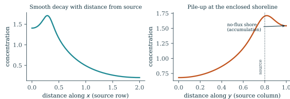
Fig. 4. (a) Computed concentration along the source row, showing smooth decay with distance from the source. (b) Computed concentration along the source column, showing the rise toward, and accumulation at, the enclosed no-flux shoreline.
