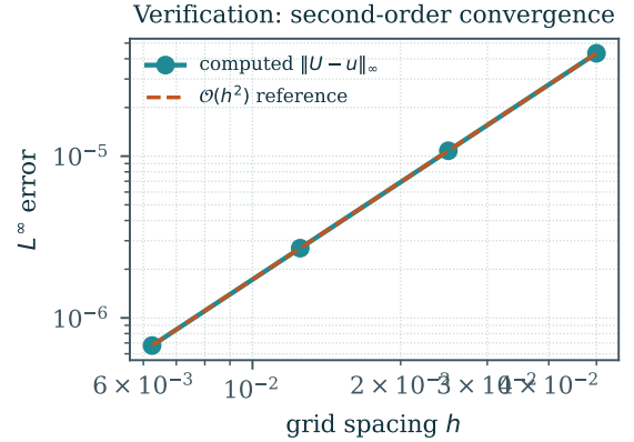
Fig. 1. Computed L^\infty error versus grid spacing h (log–log). The measured error tracks the \mathcal{O}(h^2) reference line, confirming second-order convergence of the scheme against the exact solution (7).
