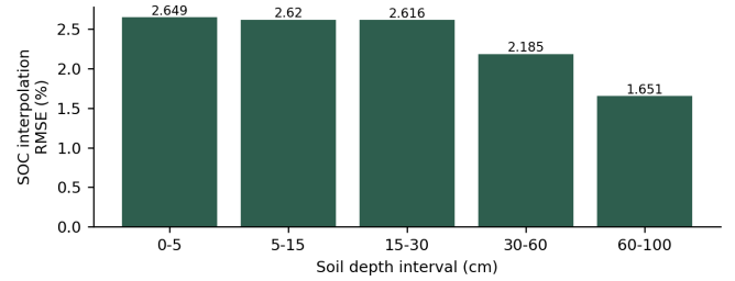
Fig. 5. National-scale SOC interpolation RMSE by depth [1].
