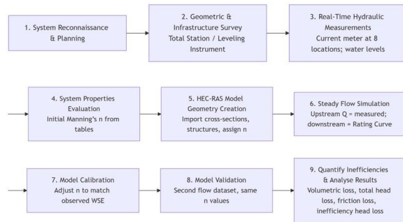
Fig. 2. Overall field measurement, modelling and inefficiency-analysis workflow.
