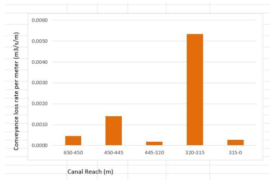
Fig. 5. Conveyance loss rate along the canal sections.
