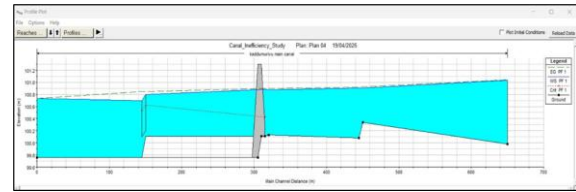
Fig. 6. HEC-RAS longitudinal profile after calibration.
