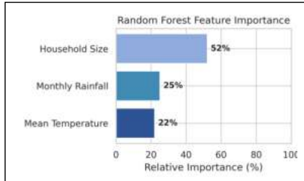
Figure 6. Relative Importance (%) of the Primary Water Demand Drivers from Stage 1 Random Forest.
