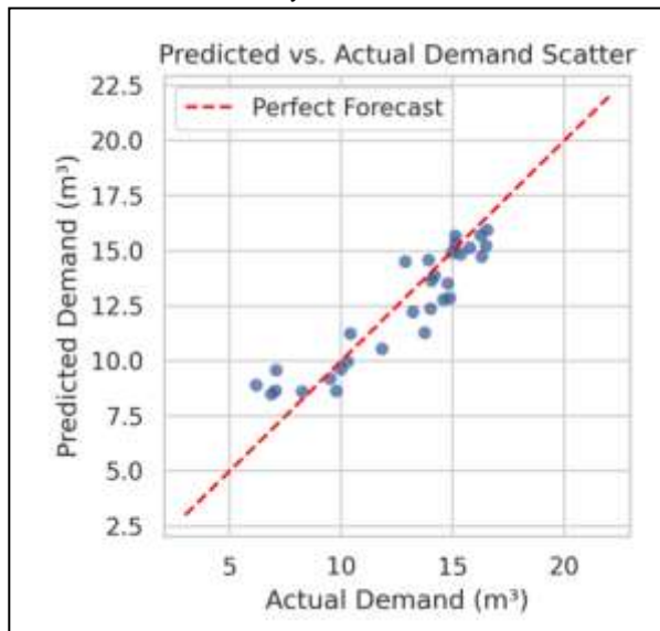
Figure 7. LSTM-Predicted Forecast versus Observed Monthly Water Demand.
