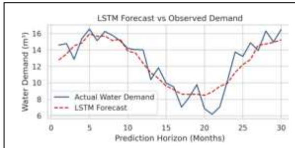
Figure 7. LSTM-Predicted Forecast versus Observed Monthly Water Demand.
