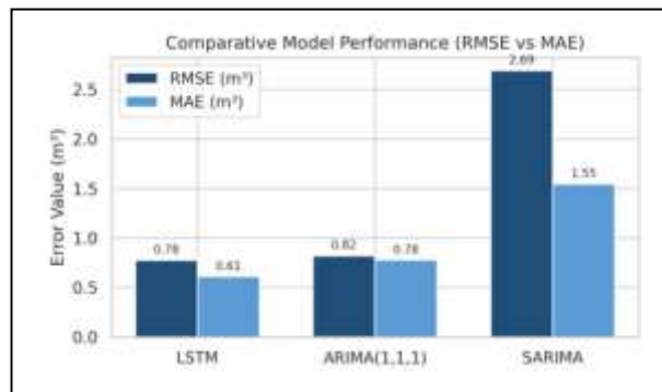
Figure 9. Bar chart comparison of RMSE and MAE across LSTM, ARIMA, and SARIMA Models.
