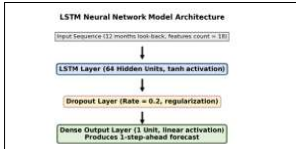
Figure 3. Structural architecture of the proposed LSTM neural network for water demand forecasting.
