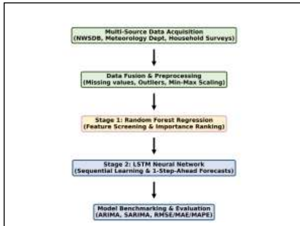
Figure 1. Methodology Flow Chart of the Proposed Joint Machine Learning Framework.
