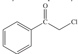
chloroacetophenone
