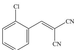
o-chlorobenzylidene malononitrile
