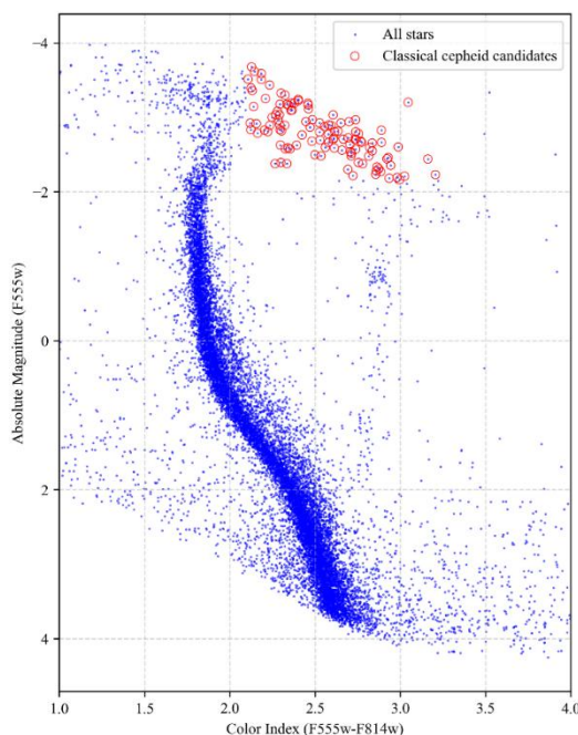
Figure 44 - Colour Magnitude Diagram of NGC 1866 with Instability Strip Stars marked in red. The Plot of V-I (F555w-F814w) Colour index vs Absolute magnitude of V (F555w) band for Globular Cluster NGC 1866
