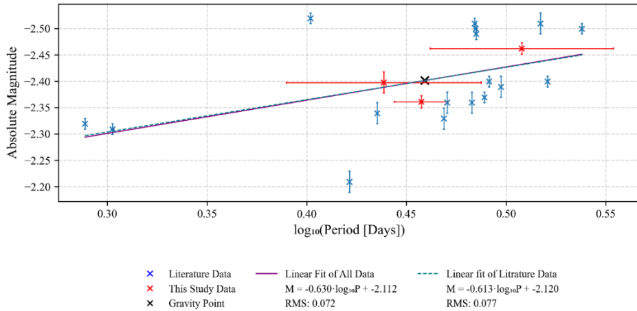
Figure 45 - Plot of Absolute Magnitude Vs \log_{10}(\text{Period}) for Cepheid Variables in NGC 1866 with linear fitting for P-L relation.
