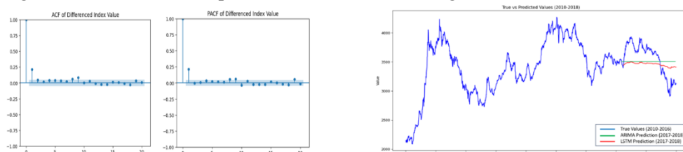
Figure 2: Results of the predicted values from the ARIMA-LSTM model
