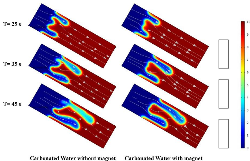
Figure 1. Spatial-temporal evolution of fingering instability of carbonated water injection at T = 25 S, T = 35 S, and T = 45 s for an angle 30^\circ .
