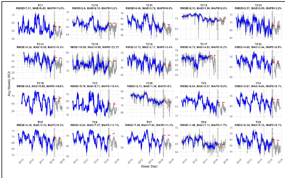
Figure 2: HES fitted models and forecasted WQI values for each monitoring site.
