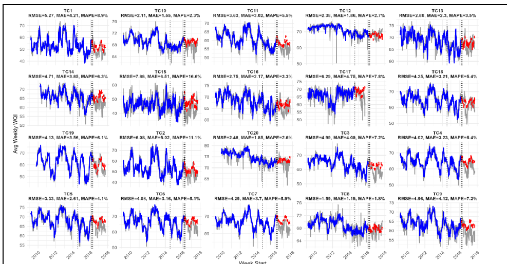
Figure 3: H-WES fitted models and forecasted WQI values for each monitoring site.
