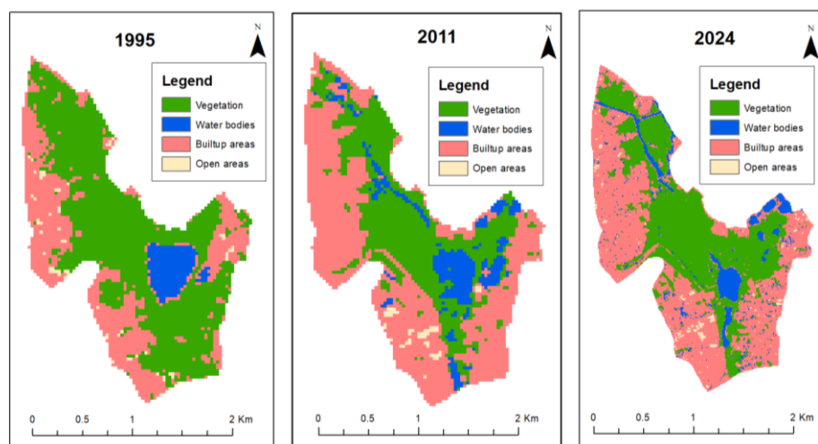
Figure 32: Spatial and temporal variation of Land Use and Land Cover (LULC) changes in Bellanwila-Attidiya Wetland (1995-2024)
