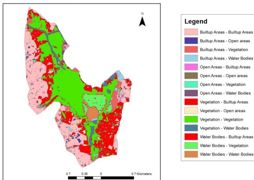
Figure 33: Change detection analysis of Bellanwila-Attidiya Wetland (1995-2024)
