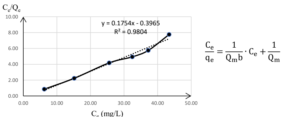
Figure 5: Langmuir Plot for LAS Adsorption onto DWTS
