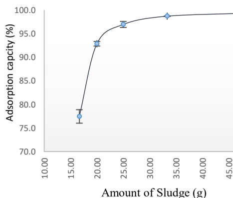
Figure 1: Adsorption capacity with different amounts of sludge (0 mm < 3.2 mm)
