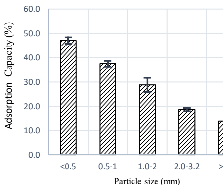
Figure 21: Adsorption capacity with different sludge particle sizes
