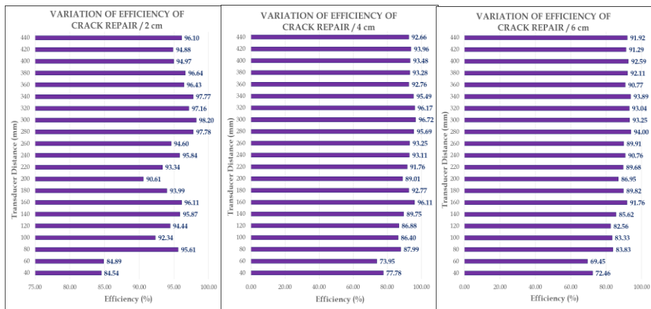
Figure 3: Efficiency of crack repair for 2cm, 4cm and 6cm crack depths, respectively
