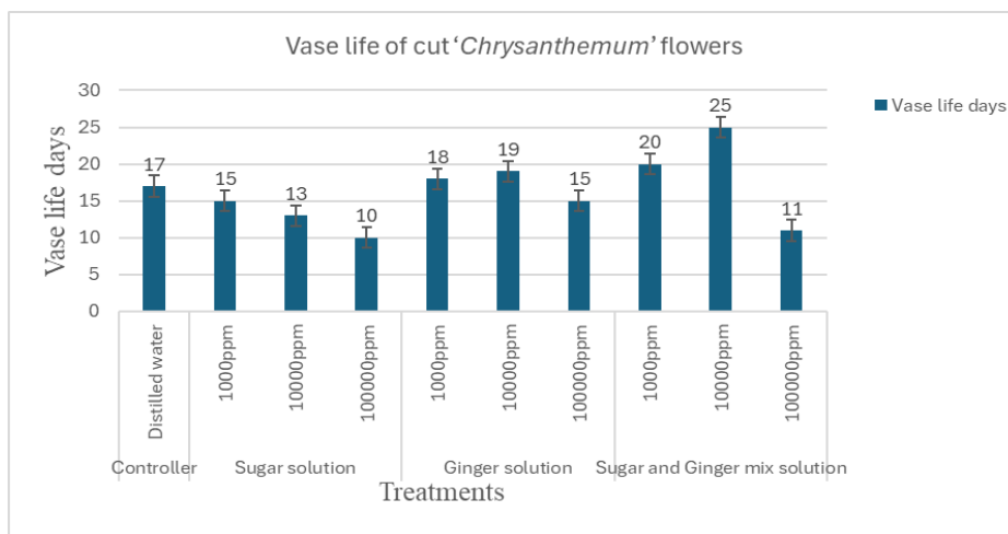
Figure 1: Effect of treatments on vase life of cut Chrysanthemum flowers
