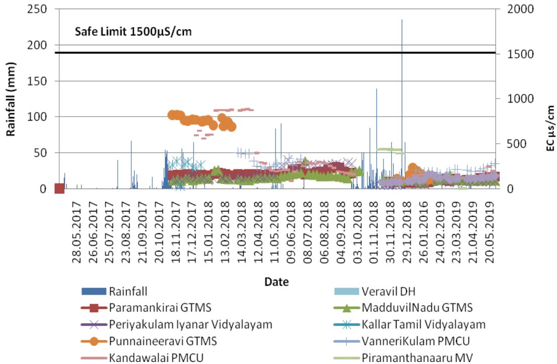
Fig. 14. Temporal variation of Electrical Conductivity in rainwater harvesting tank water
