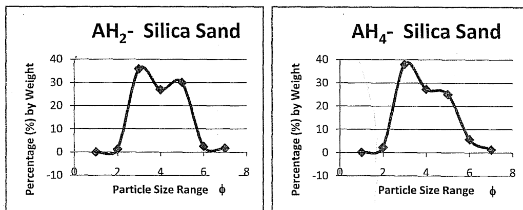
Fig. 2: Representative grain size distributions of the sand samples taken from two augur holes, which indicate a similar composition being composed of bi-modal distribution
